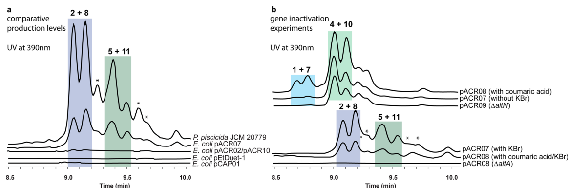
Figure 2. (a) LCMS UV trace showing comparative production levels of aliterochromide molecules in the native producer P. piscicida JCM 20779 and two E. coli heterologous expression constructs (pACR07 and pACR02/pACR10) alongside empty vectors. Bromoaliterochromide A (2)/bromoaliterochromide A' (8) are detected in all three, albeit at levels 3-fold and 60-fold less than the native producer for the expression in E. coli with pACR07 and pACR02/pACR10 respectively. (b) LCMS UV trace showing aliterochromide metabolite profiles for gene inactivation mutants of aliterochromide pathway ( \Delta altA or \Delta altN ) and feeding experiments ( \Delta altA /coumaric acid, \Delta altA /coumaric acid/KBr, pACR07/KBr, or pACR07/without KBr), relative production levels not to scale. Note: peaks labeled with an asterisk are other aliterochromide compounds.
